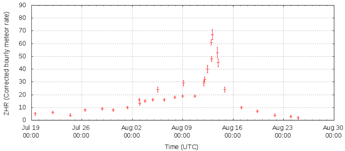
Figure 4 – Reduced hourly counts of visual meteors ( http://www.imo.net/live/perseids2014/ ).
