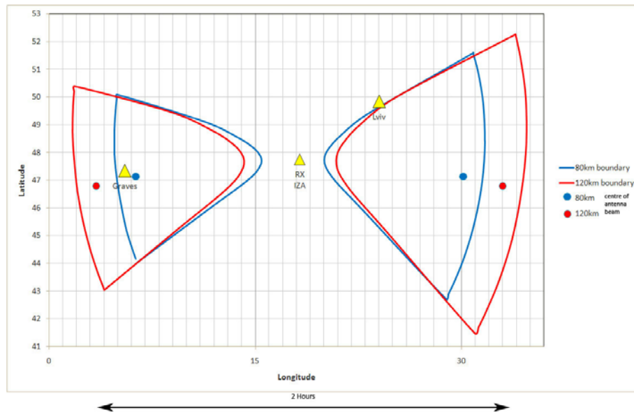
Figure 1 – Theoretical field of view of both antennas calculated for the upper (120 km AGL) and the lower (80 km AGL) boundary of detectability of radiometers.
